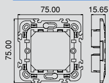
Mounting Frame 2M
