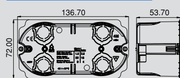
Hallow Wall Box 4M
