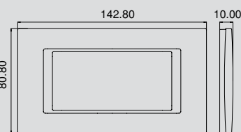
Optima 4M Frame
