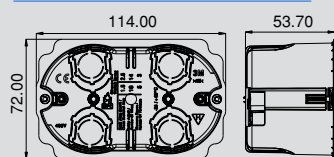
Hallow Wall Box 3M
