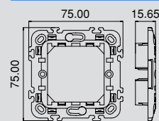
Metal Mounting Frame 2M
