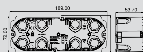
Hallow Wall Box 7M
