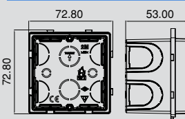
Wall Mount Box 2M
