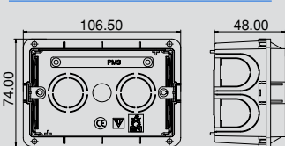
Wall Mount Box 3M
