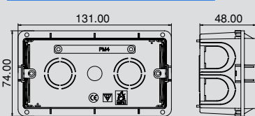
Wall Mount Box 4M
